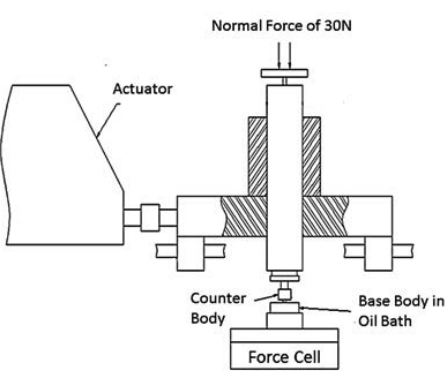
(4) Struktur des Labortribosystems und der Beanspruchungskollektive. Quelle (4–6): D. Stickel, The Influence of Surface Finish on the Localized Dissipation of Frictional Power at Ultra-Mild Wear. PhD-Thesis, Materials Science and Engineering, University of Duisburg-Essen, Duisburg, Germany, DuEPublico ID 39526, 2015.
